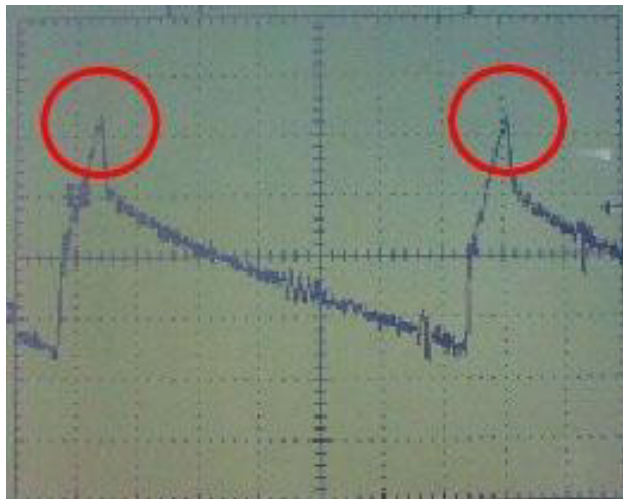
Figure 4: The shape of the waves using a short-side terminal resistor with the switching noise
