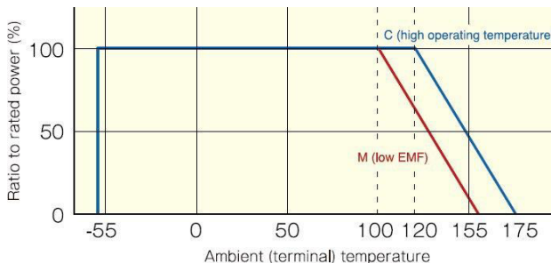
Figure 3: Curve shows higher derating point
